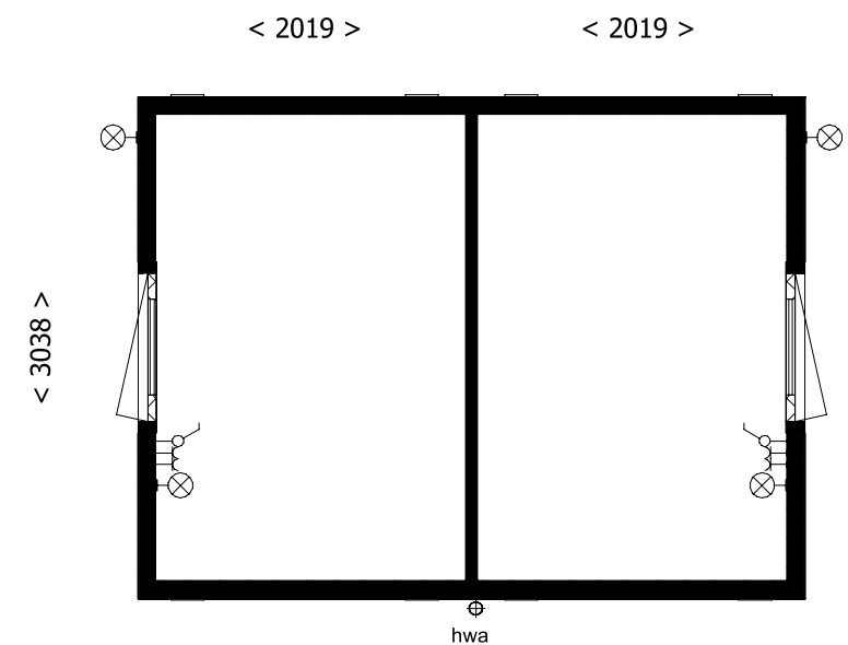
V0 = begane grond (Peil) 1 : 50
